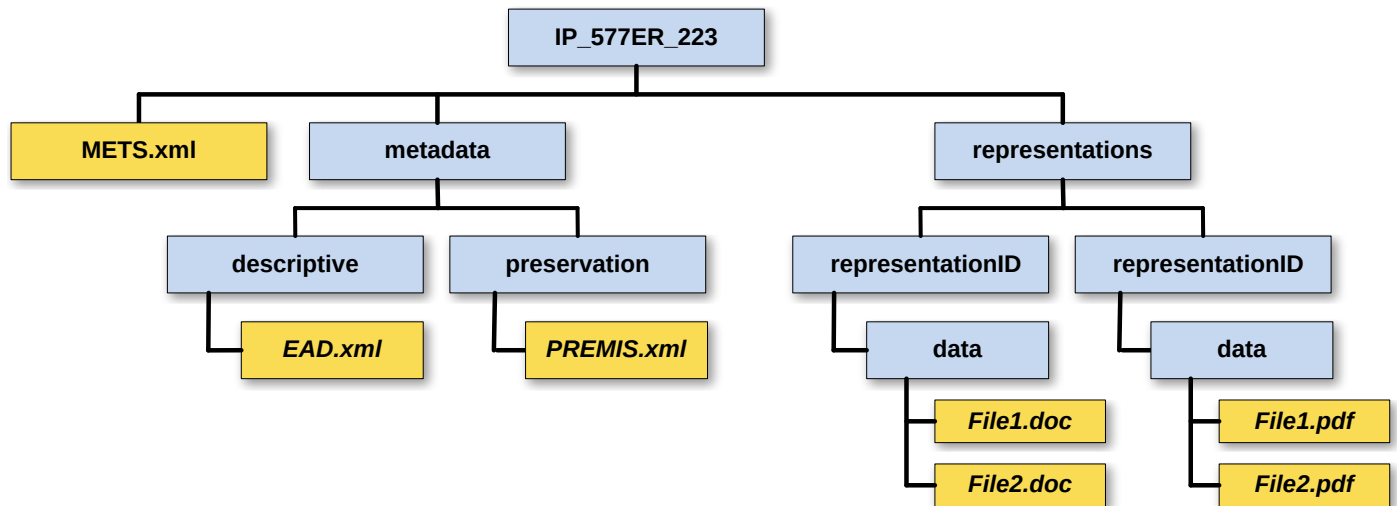
Figure 9: A simple CSIP structure example.
